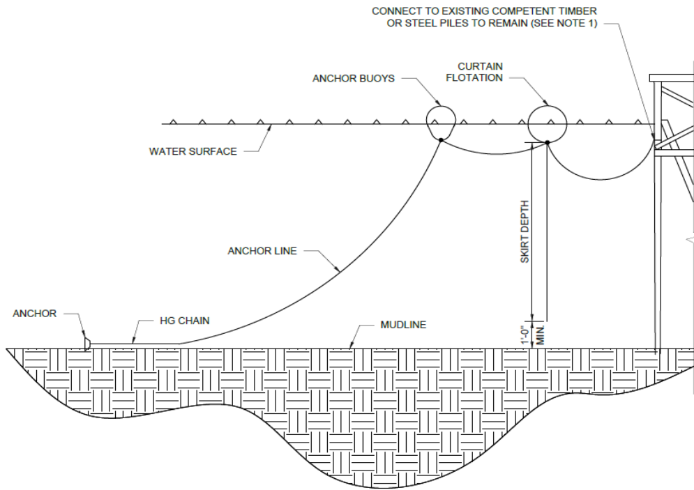
TURBIDITY CURTAIN DETAIL NOT TO SCALE
